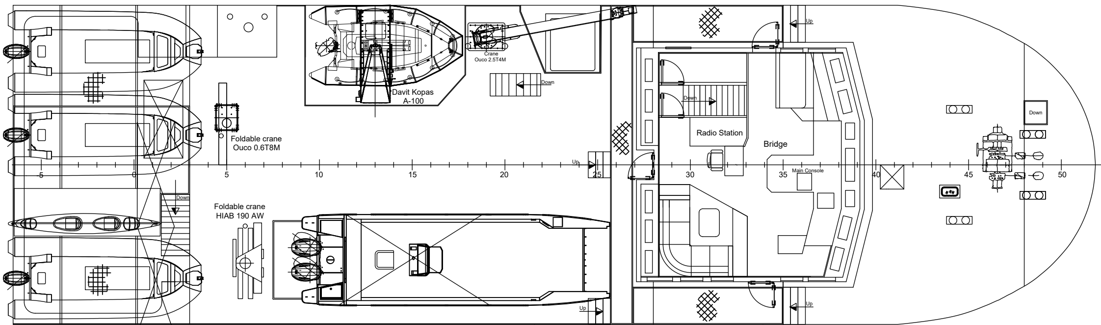
BOAT DECK
