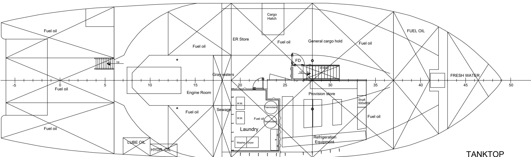
TANKTOP
