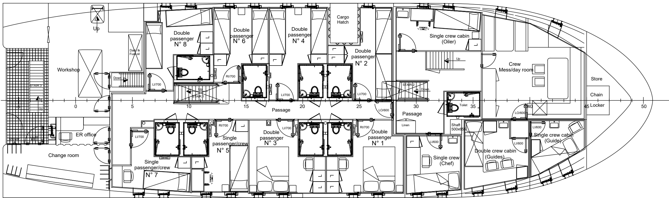
MAIN DECK
