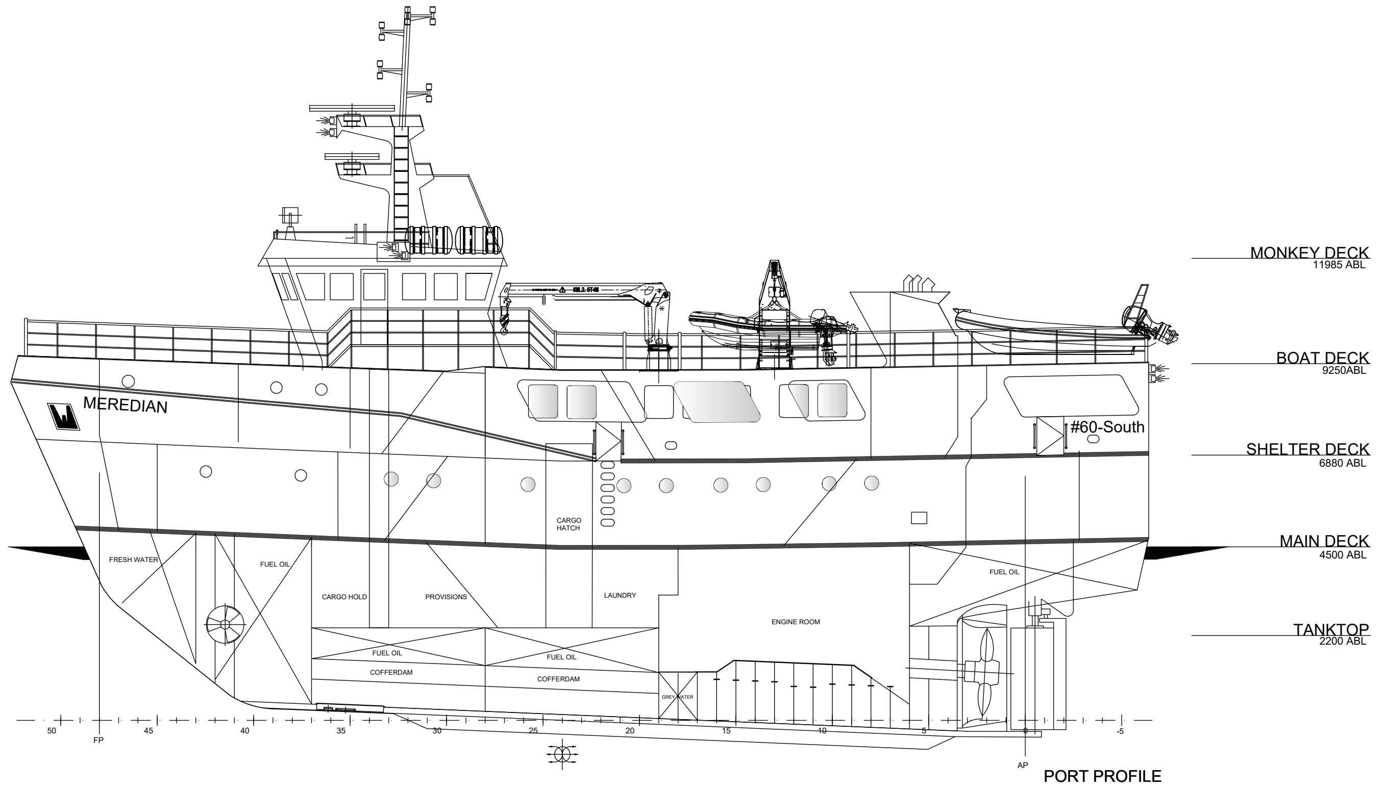
PORT PROFILE
