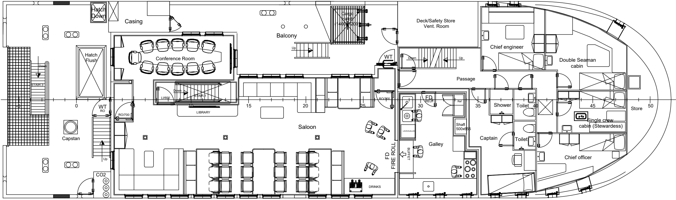
SHELTER DECK
