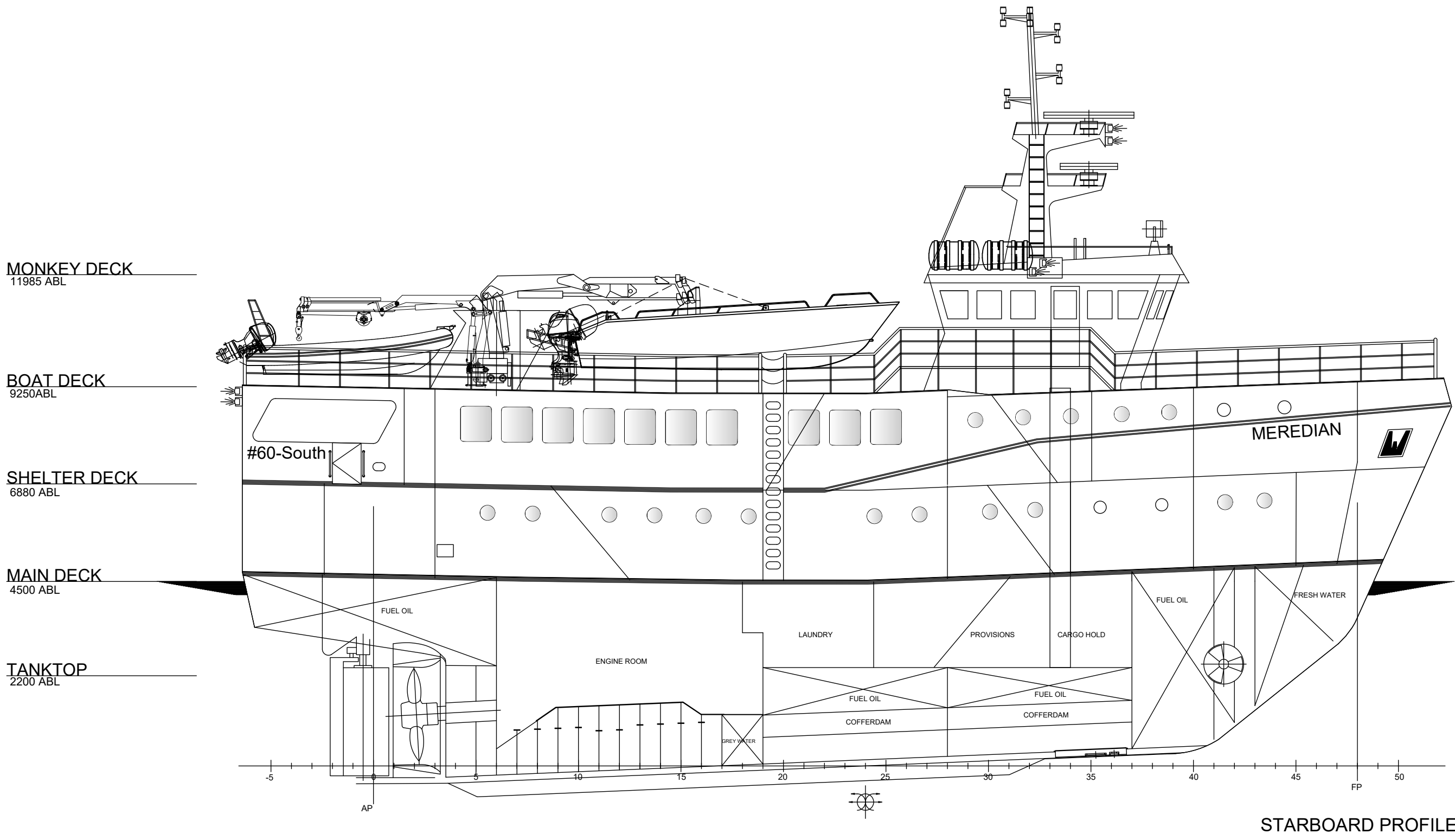
STARBOARD PROFILE
