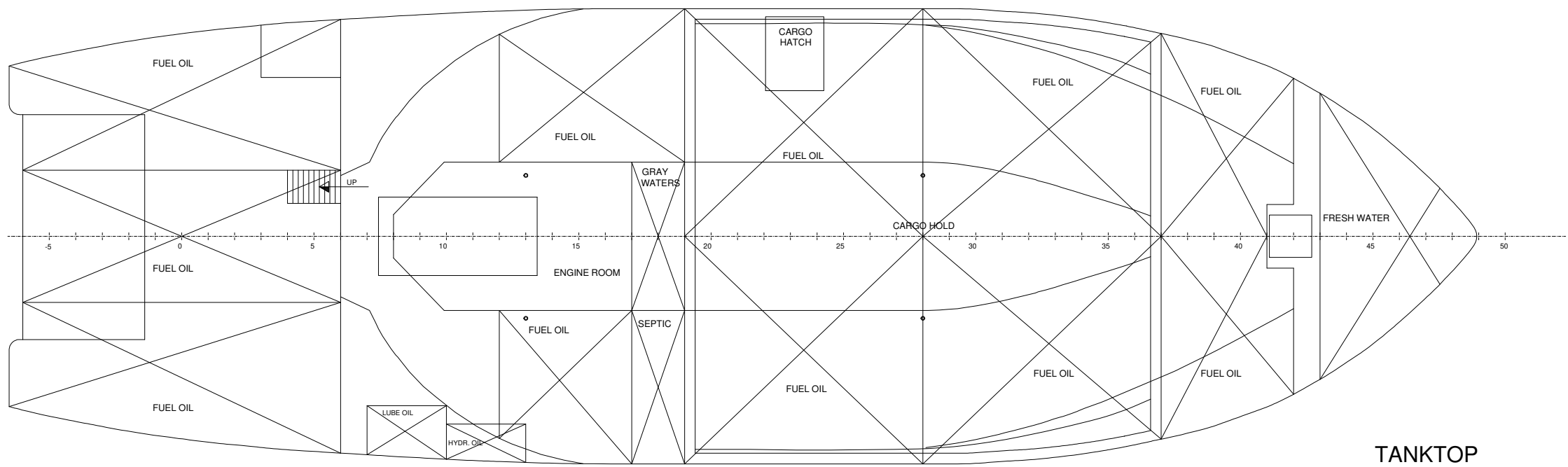
TANKTOP
