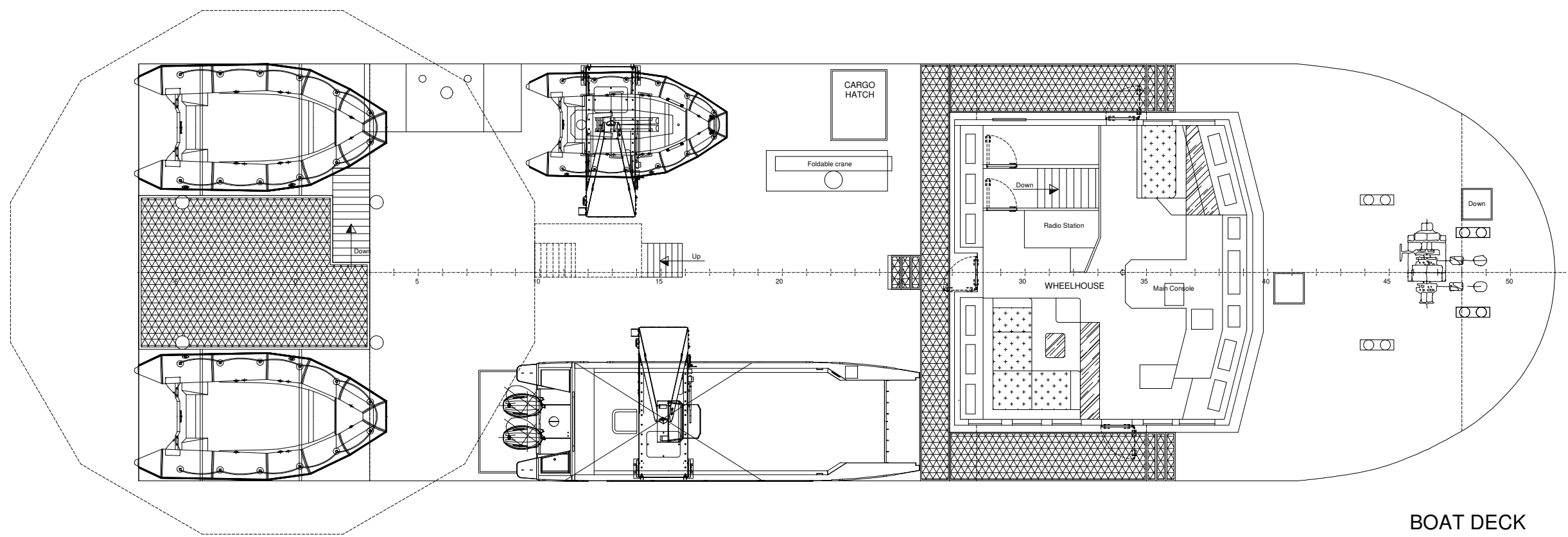
BOAT DECK
