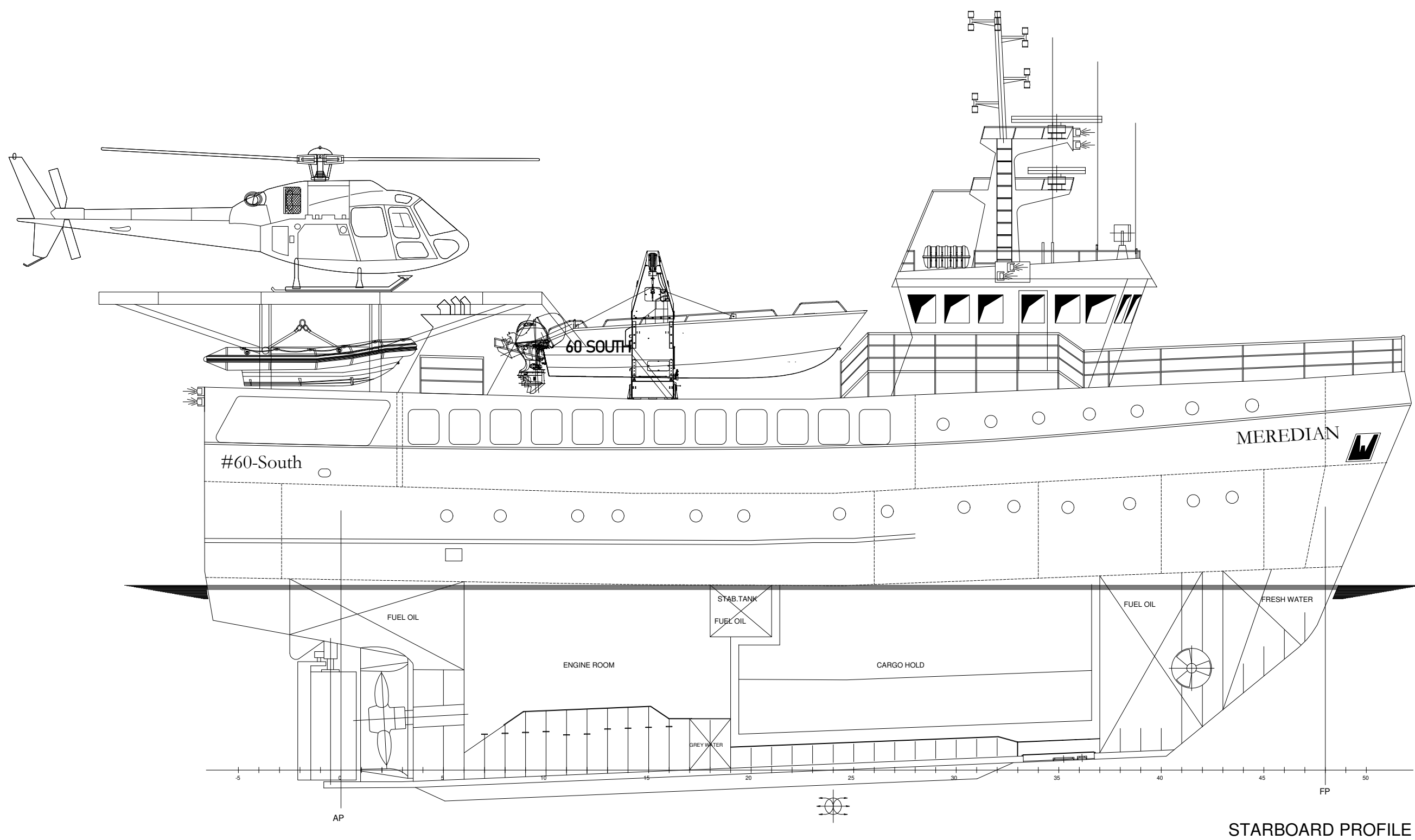
STARBOARD PROFILE
