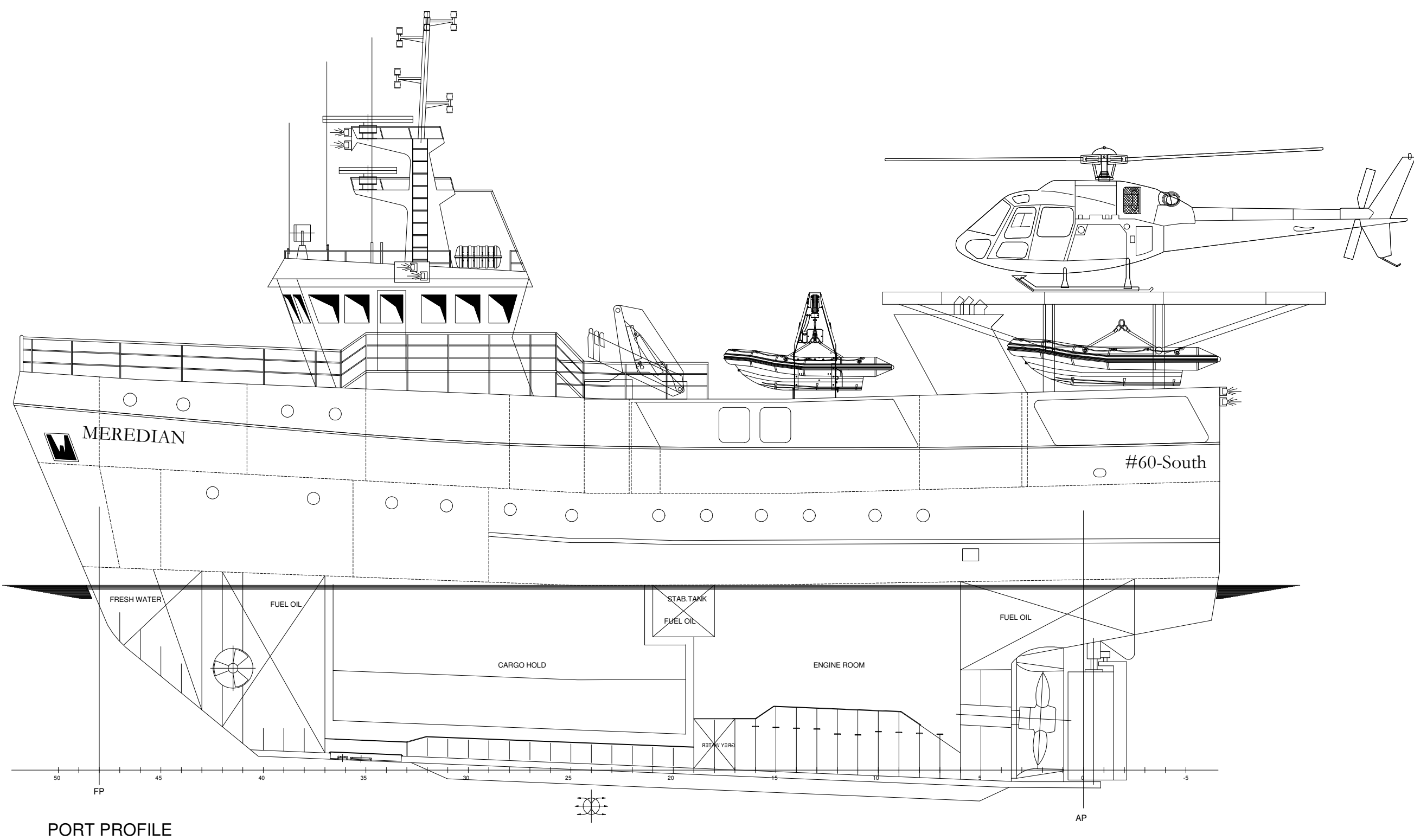
PORT PROFILE
