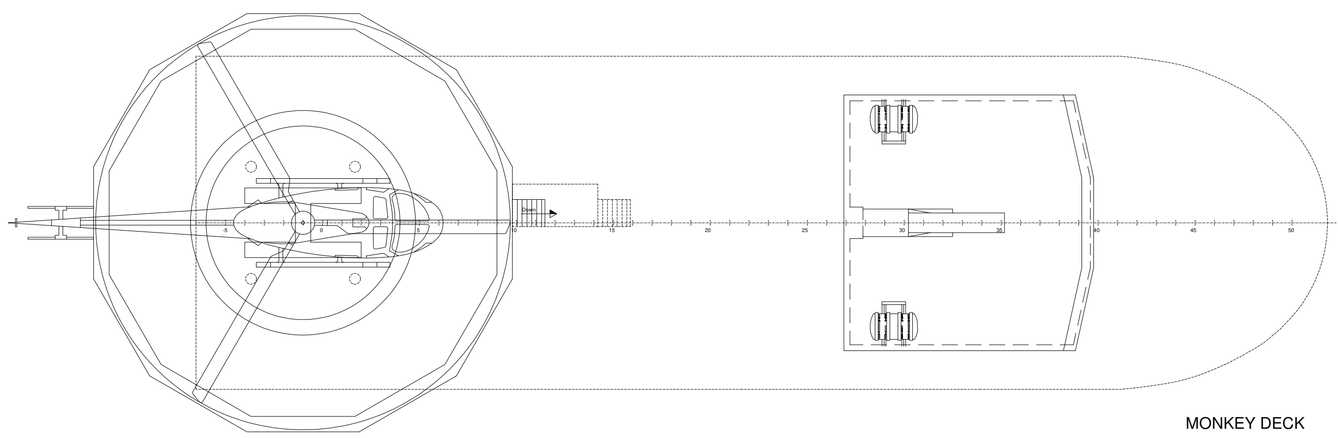
MONKEY DECK
